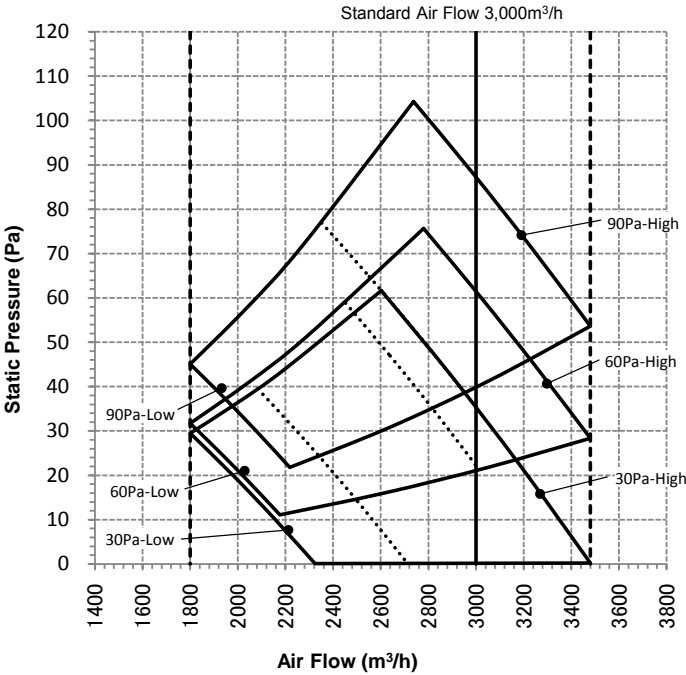
AP0276 type
