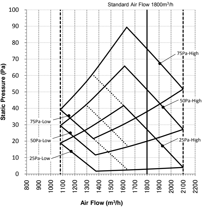
AP0186 type
