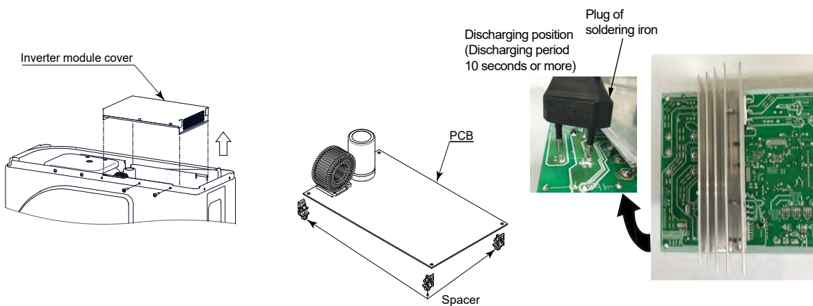
Fig. 11-5 (RAS-07, 10, 13J2AVSG-E)
